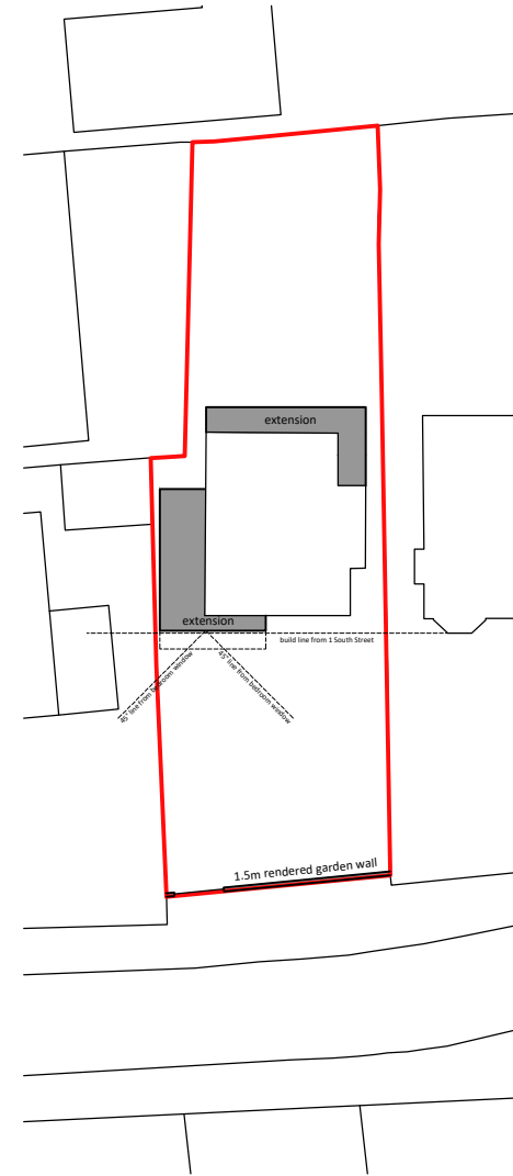
Proposed Site Block Plan 1:500
